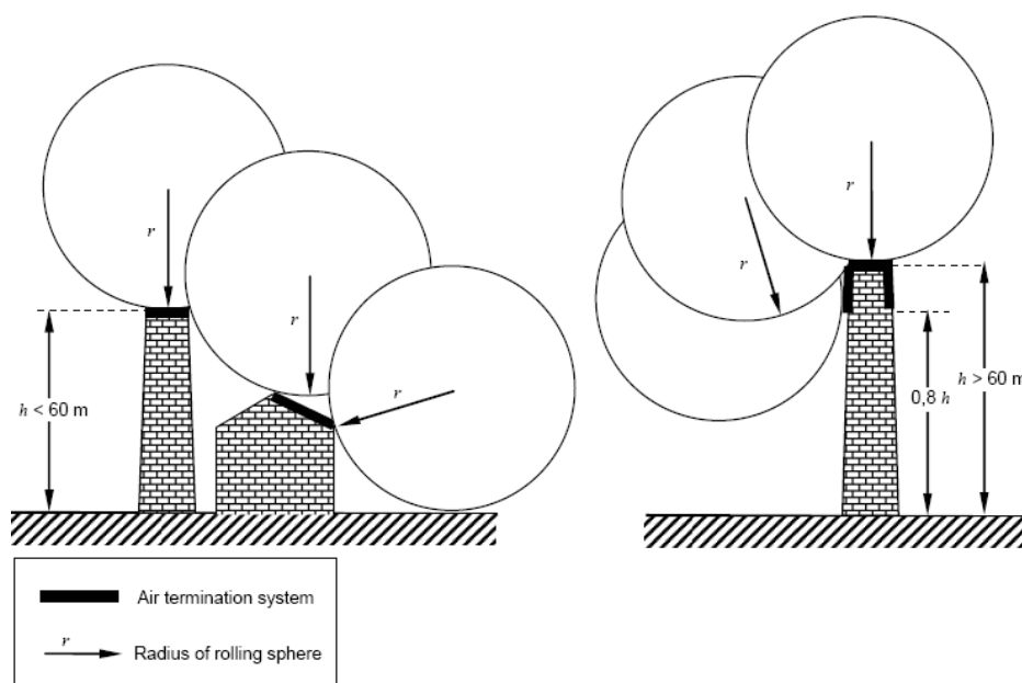
Figure 8-3 Design of an air-termination system according to the rolling sphere method
