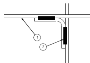
Figure 8-8 Welded joints of reinforcing rods in reinforced concrete
