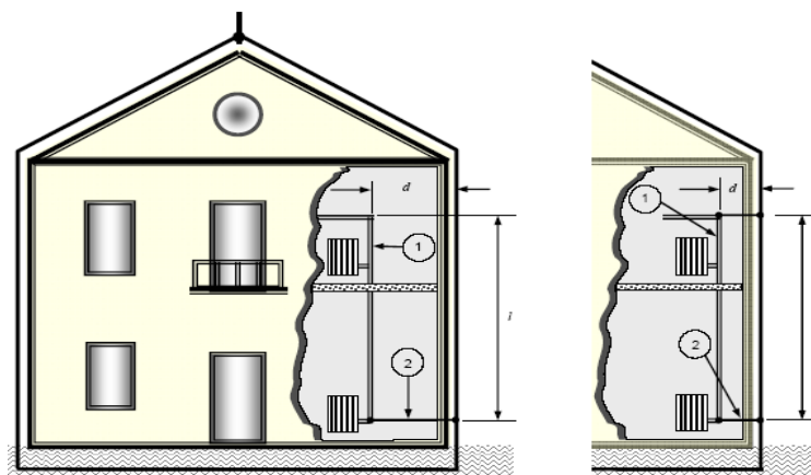
Figure 8-7 Calculated separation distances
