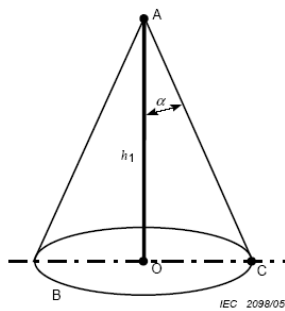
Figure 8-2 Volume protected by a vertical air-termination rod
