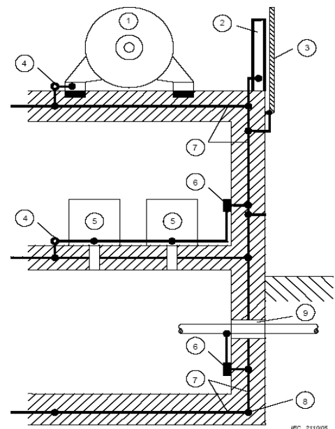
Figure 8-6 Equipotential bonding in a structure with a steel reinforcement
