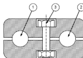
Figure 8-9 Circular conductor to a reinforcing rod
