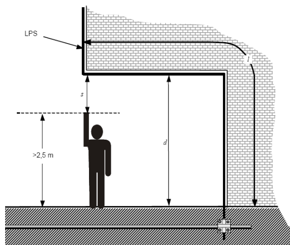
Figure 8-5 LPS design for a cantilevered part of a structure
