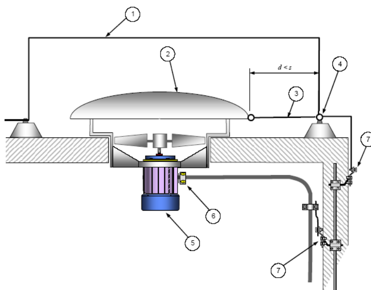
Figure 8-4 Metallic roof fixture protected against direct lightning interception, connected to air-termination system
