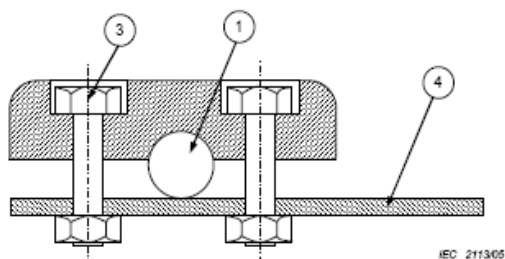
Figure 8-10 Solid tape conductor to a reinforcing rod
