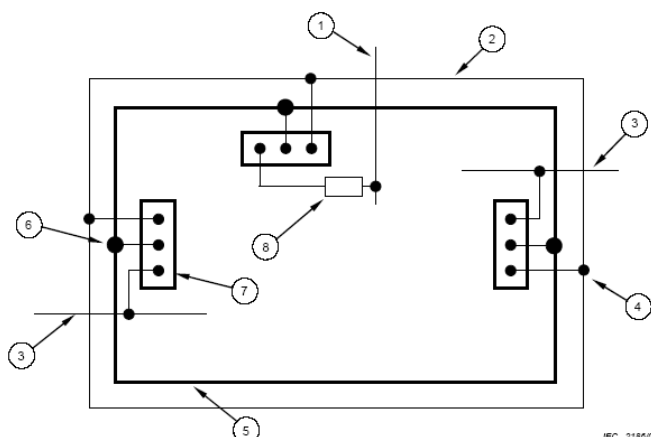
Figure 8-11 Example of bonding arrangement
