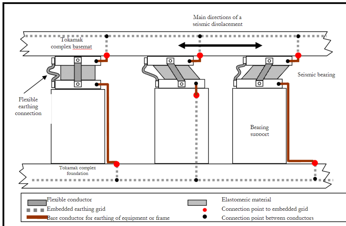
Figure 6-4 Earthing of Tokamak Basemat with Flexible Interconnections
