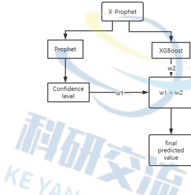
Figure 4: The structure of improvement prophet X-Prophet
