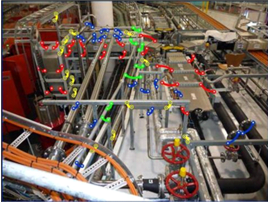
Figure 8-5 Examples of bonding natural metalwork, on an existing synchrotron, #1.
