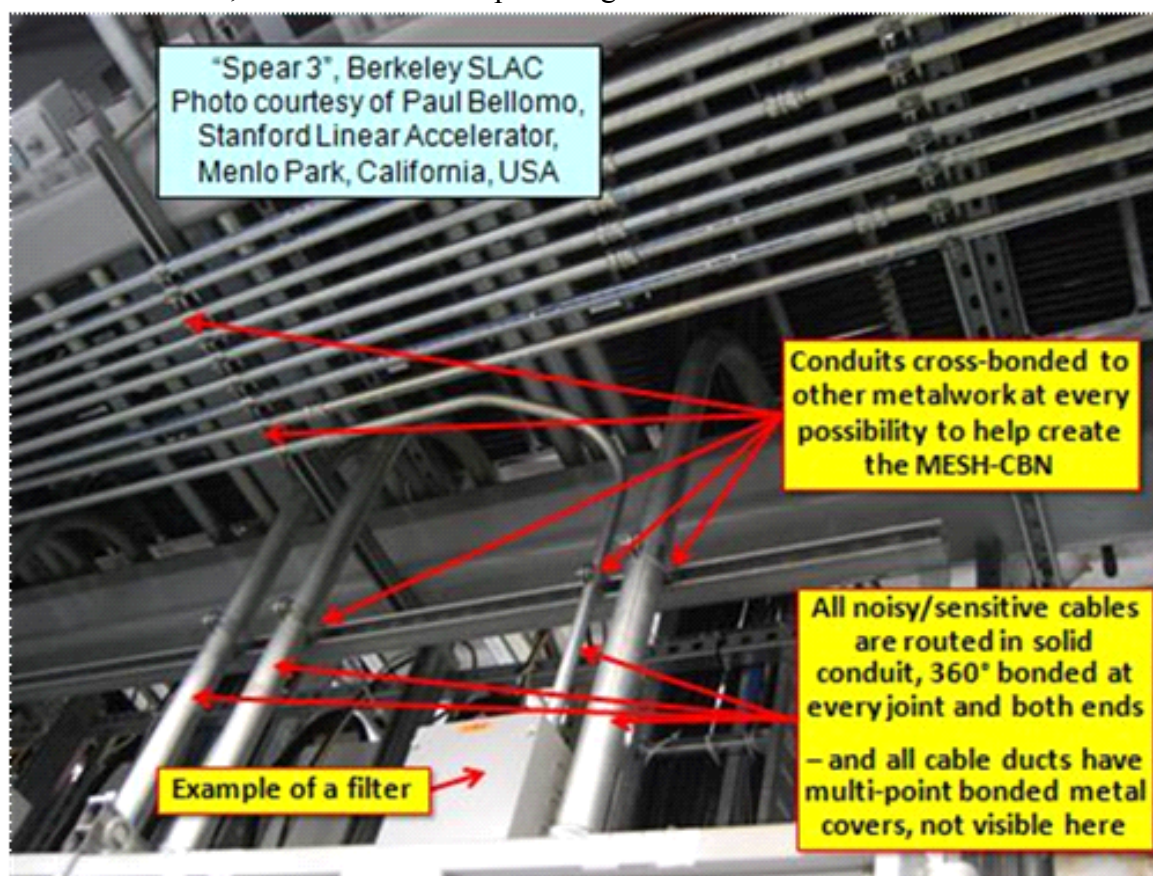
Figure 13-1 Example of a well-constructed system using solid circular conduit and covered ducts.
