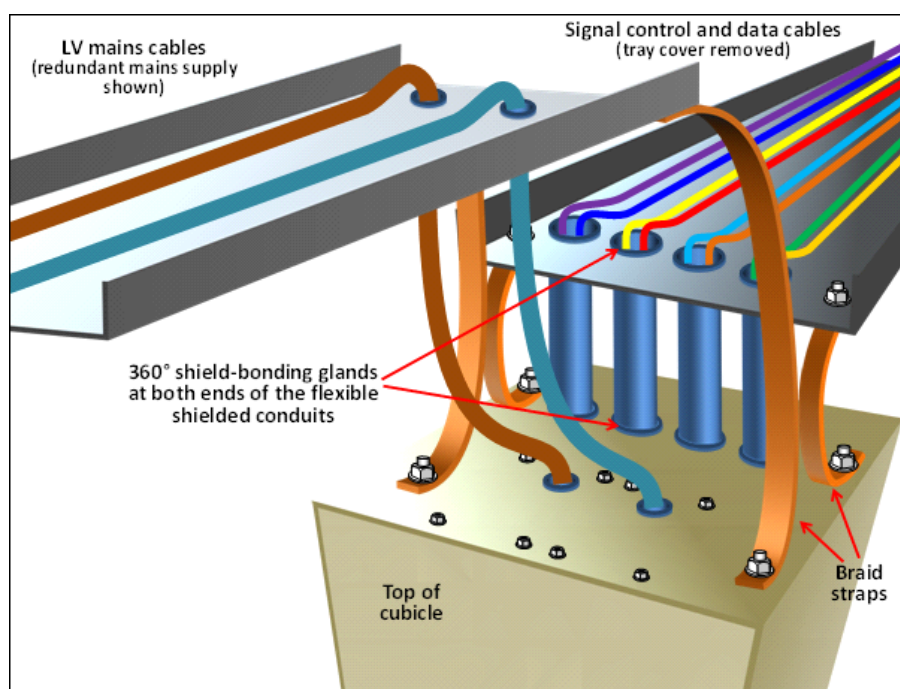
Figure 5-3 More details on electrically bonding all cable trays and terminating all cable shields to the equipment connection panels at both ends.
