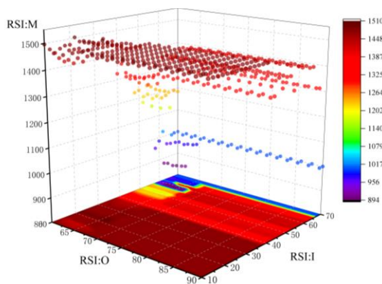
Figure 5: fixed parameter optimization
