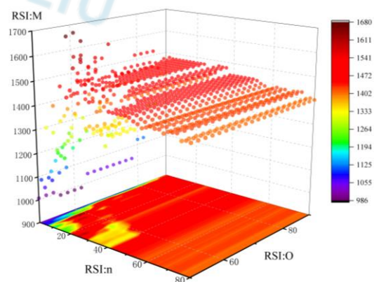
Figure 6: Fixed parameter optimization
