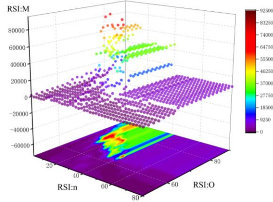
Figure 3: Fixed parameter optimization
